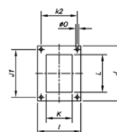
Outlet nozzle 680/790
