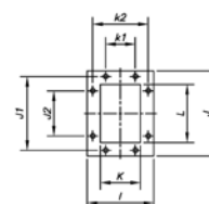
Outlet nozzle 980...1090
